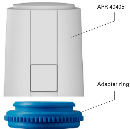
Valve actuator APR 40405 and adapter ring.
