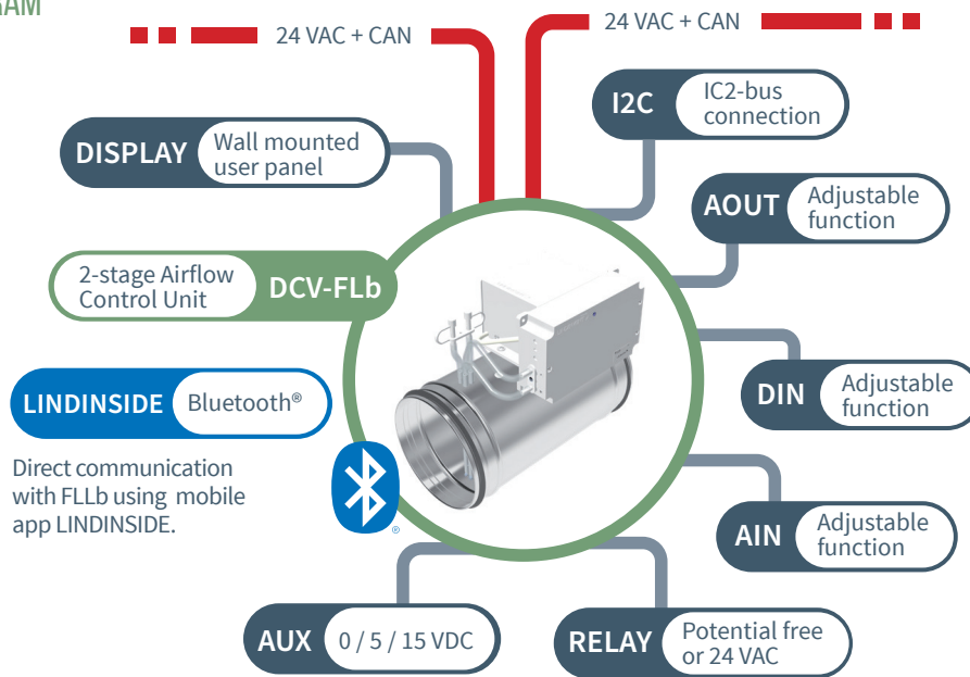
Connection diagram for FLLb. The regulator is connected to CAN and voltage fed via Lindinvent's 4-conductor cable.
