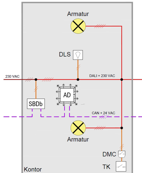
Example Operating Card with SBD2b for Addressed DALI with Wired Switch (TK).
